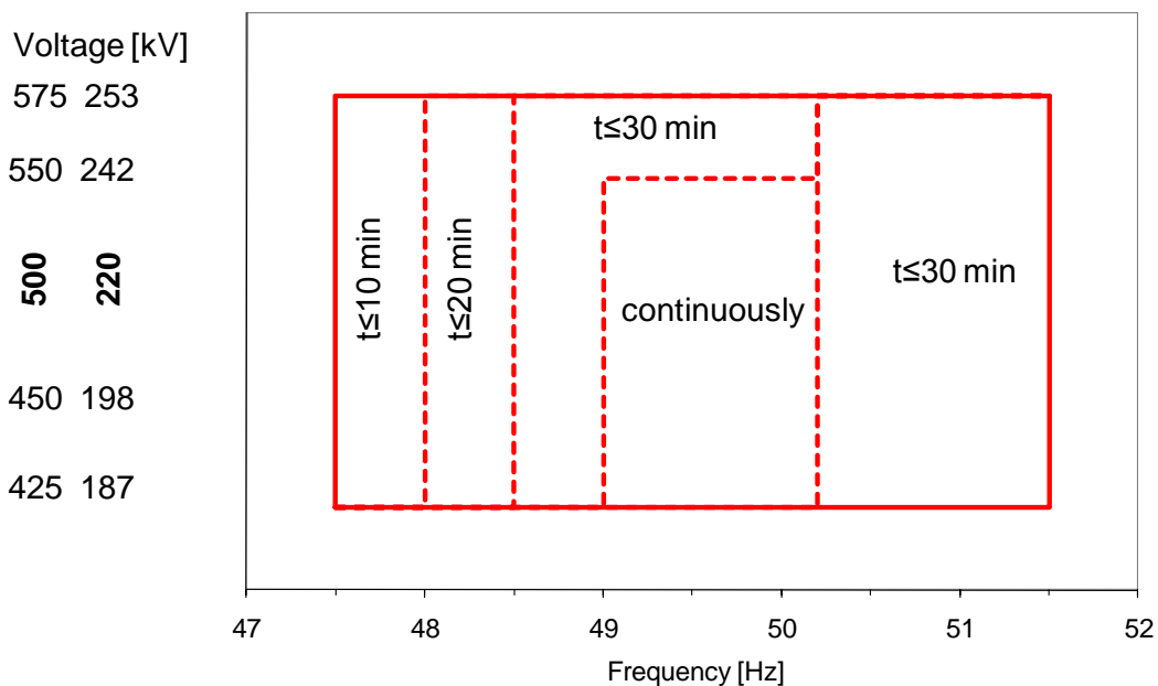
Figure 5.1: Requirements on the output power of the Wind Farm in case of grid frequency and grid voltage variations (quasi-stationary observation)
