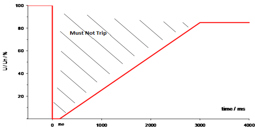
Fig. 5.4: Fault ride through profile for a Wind Farm
