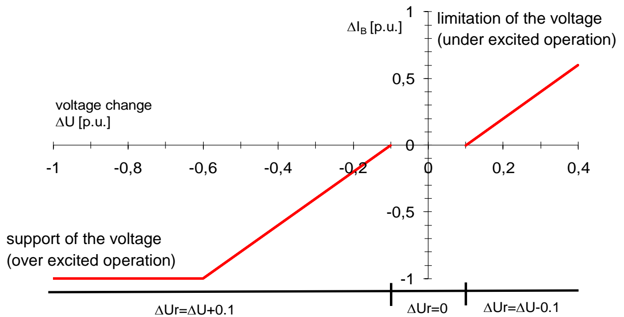
Figure 5.5: Current injection during the fault
