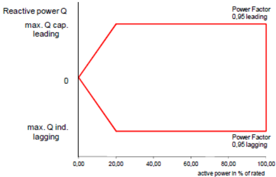
Figure 5.3: P-Q Diagram
