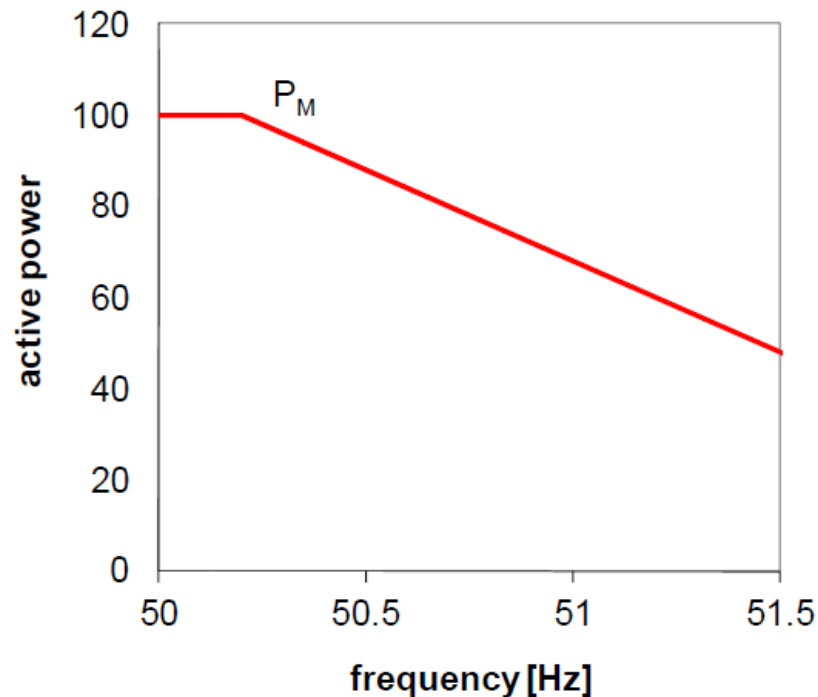
Figure 5.2: Active power reduction due to over frequency
